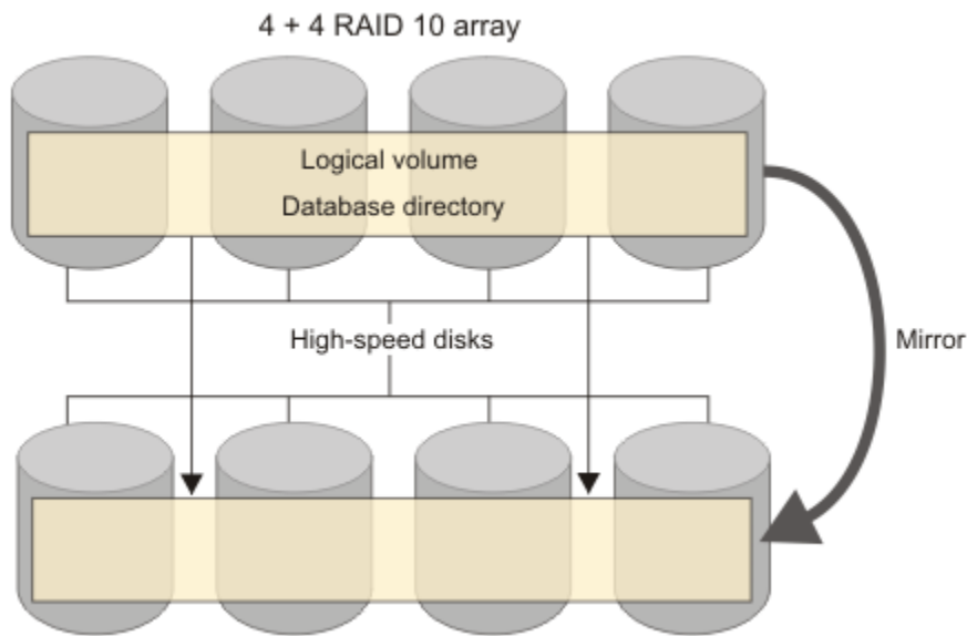
Figure 25. Database layout that uses eight disks in a RAID 10 array
